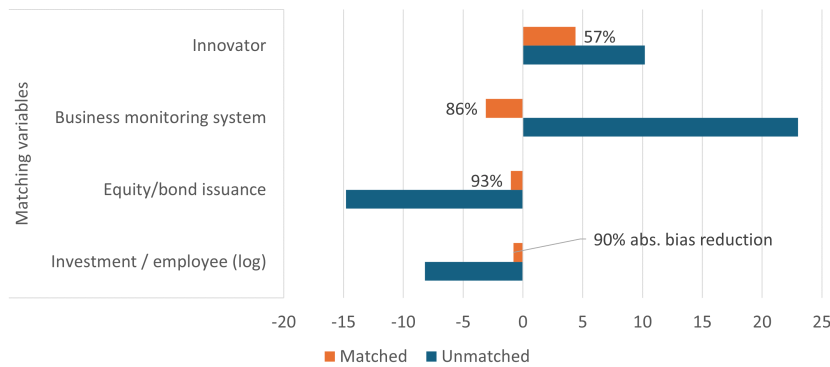
Figure 6: Balancing properties before and after matching
