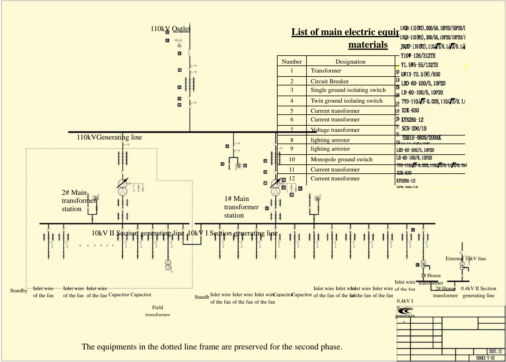
Fig.3 Main Electric Wiring Figure of the Booster Station
