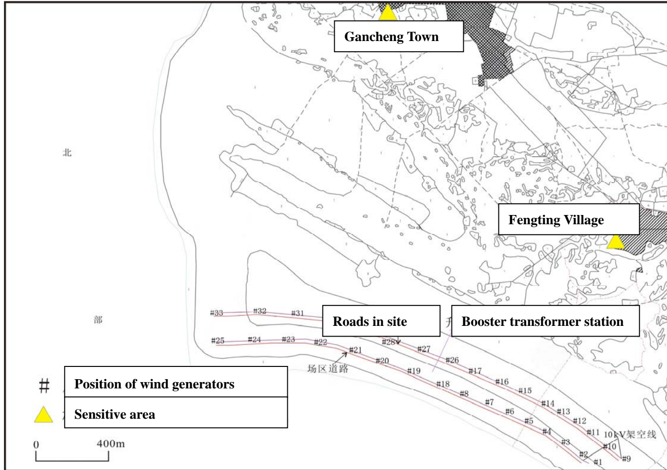
Fig.2 General Layout of the Project
