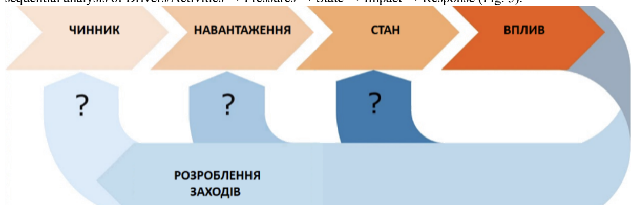
Figure 5 DPSIR conceptual model
