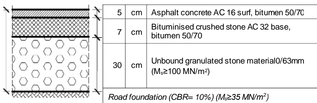
Drawing 4.7.2. Schematic section of the rigid road pavement
