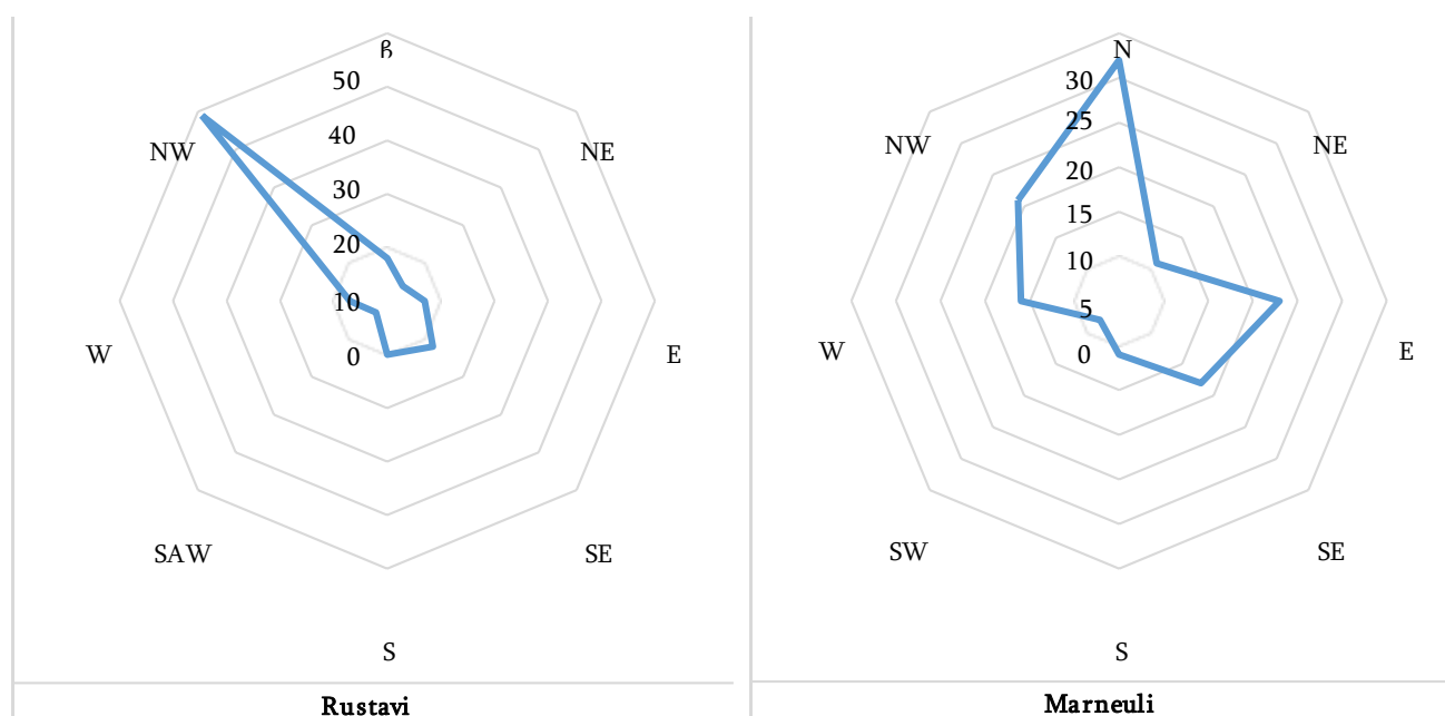
Wind rose, %:
